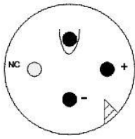
Figure 26: Power Connector – Bottom Panel
